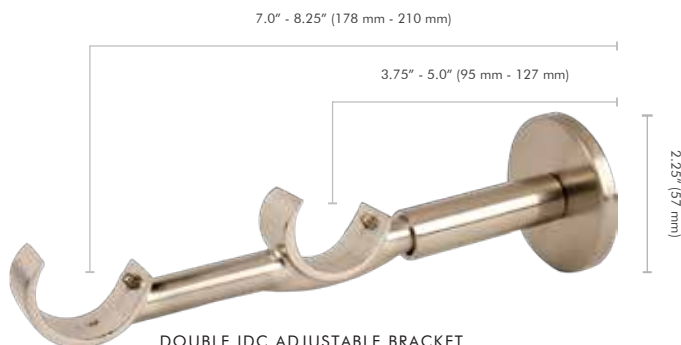
DOUBLE IDC ADJUSTABLE BRACKET SUPPORT AJUSTABLE DOUBLE IDC
